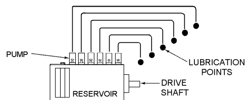
Pump-to-Point System
